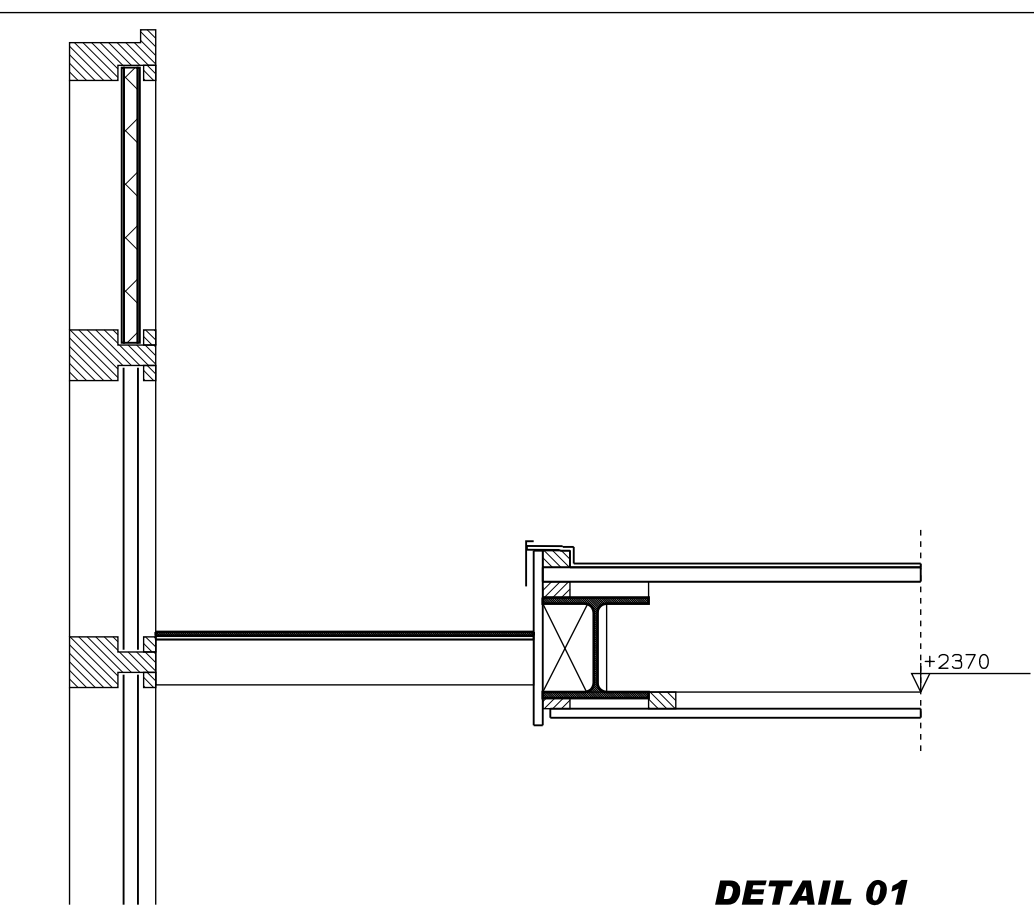
DETAIL 01
